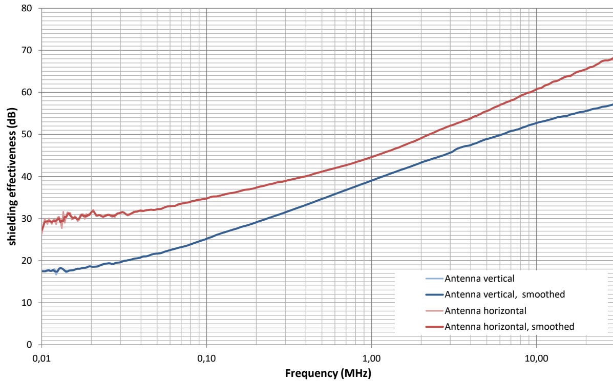
Shielding effectiveness 10 kHz - 30 MHz, Front
