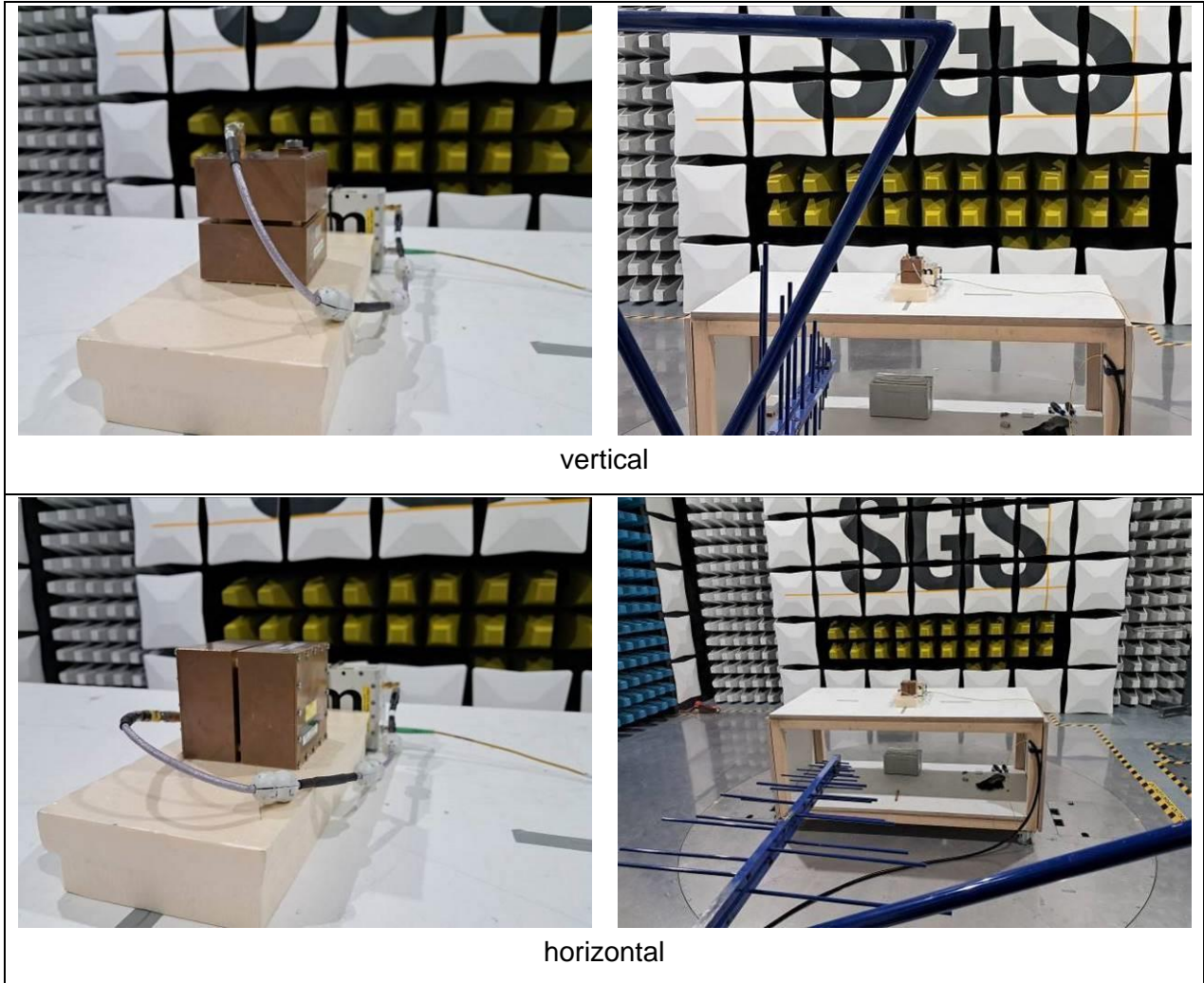
Figure 6-7: test setup reference measurements for position side
