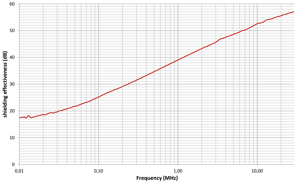
Shielding effectiveness 10 kHz - 30 MHz, Worst Case
