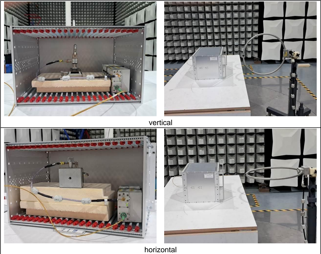
Figure 6-3: test setup 0.01 – 30 MHz
