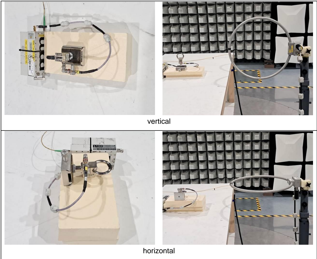
Figure 6-2: test setup reference measurements for position side
