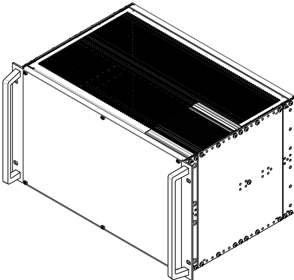
Figure 4-1: EUT
