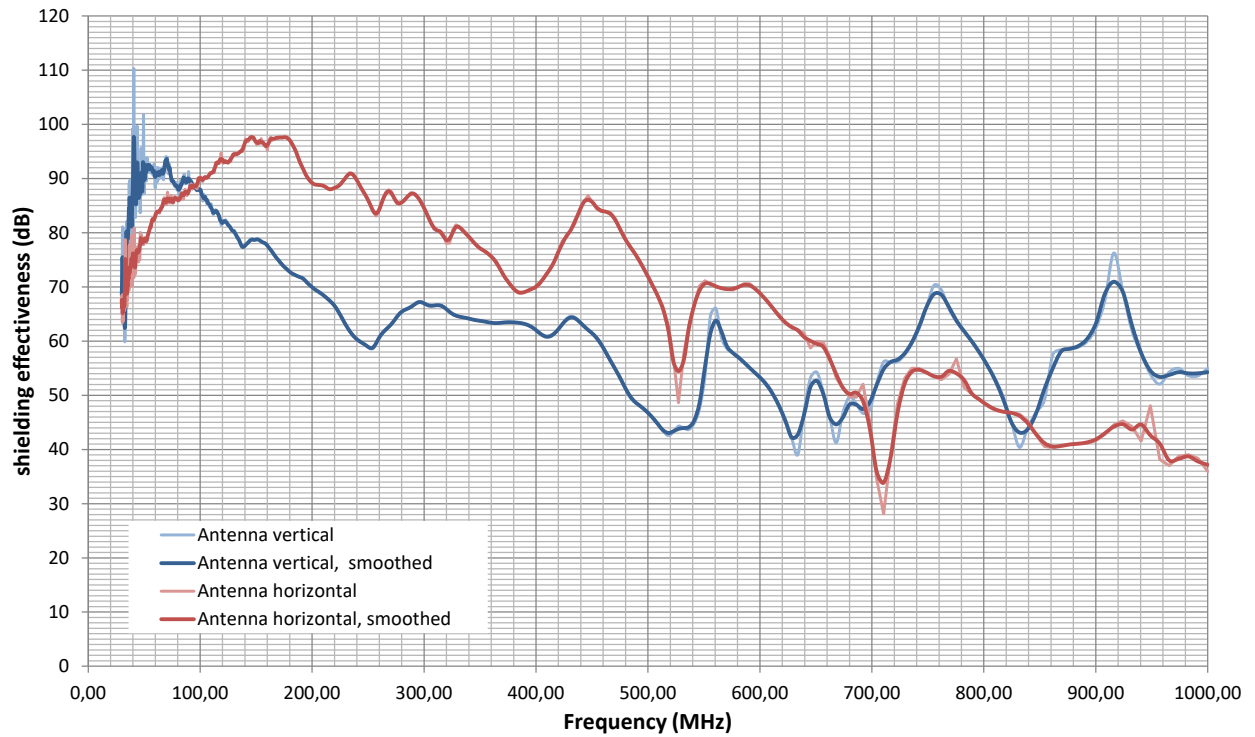
Shielding effectiveness 30 - 1000 MHz, Front
